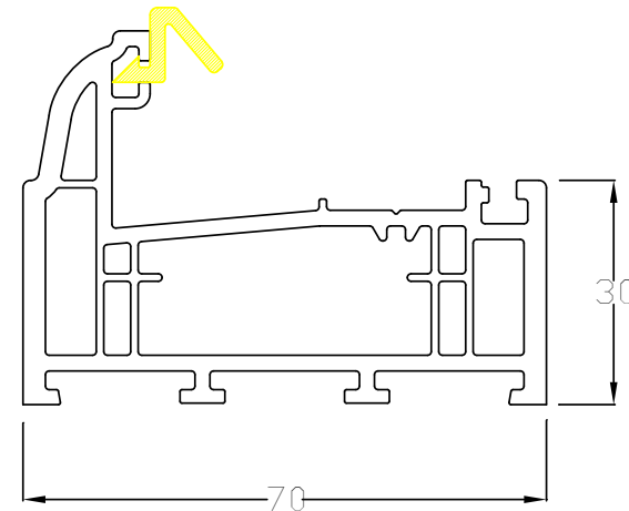
SLIMELINE FRAME
